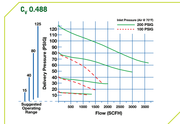
ELC4 FLOW DATA - EDGE Series-Liquid Cylinder
